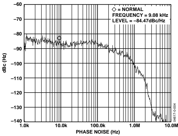
Figure 4. Phase Noise Response— DV_{DD} = 3.0 V , I_{CP} = 0.86 mA , I_{VCO} = 2.0 mA , F_{OUT} = 315 MHz , PFD = 3.6864 MHz , PA Bias = 5.5 mA
